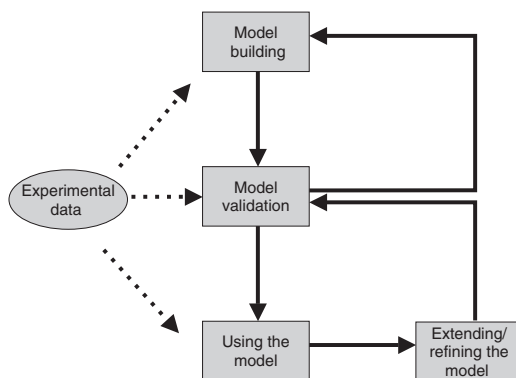
Figure 12.3 Flow diagram to show the steps in building a model. Once a model has been built, it is tested against experimental data. If the model does not agree well, then the modeler goes back to the model-building stage. Otherwise, the model can be used and then extended further as more knowledge becomes available.
