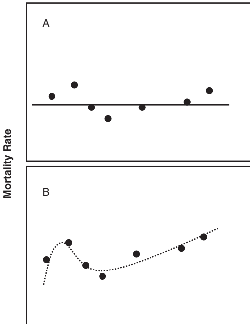
Figure 9.1 Misleading inference of no senescence caused by elevated risk-taking during dispersal or territory acquisition. A. Regression from points sampled. B. Underlying mortality pattern. • Ages sampled. Dashed line = actual adult mortality trajectory, solid line = inferred mortality trajectory from 5 sampled ages.
